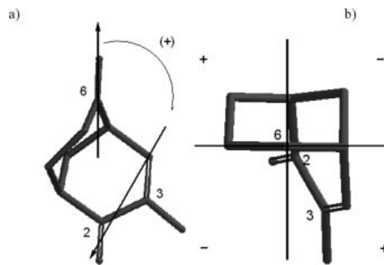
Figure 2. (a) Distorted cyclohexenone chair conformation (in front) and angle between planes containing chromophores in triketone 4 ; (b) Division of the C-6 carbonyl group in triketone (+)- 4 into octants.
