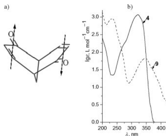
Figure 3. (a) The orientation of dipoles in the minimized structure of bis(enone) 9 ; (b) UV spectra of triketone 4 (—) and bis(enone) 9 (---).
