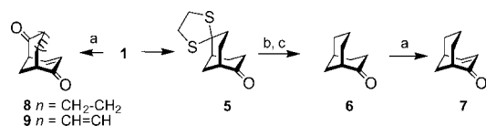
Scheme 2. (a) \text{PhIO}_2 , \text{PhSeSePh} , \text{TsOH} (cat.), toluene, reflux; (b) \text{Ra-Ni} , \text{EtOH} , reflux; (c) Jones reagent, room temp.
