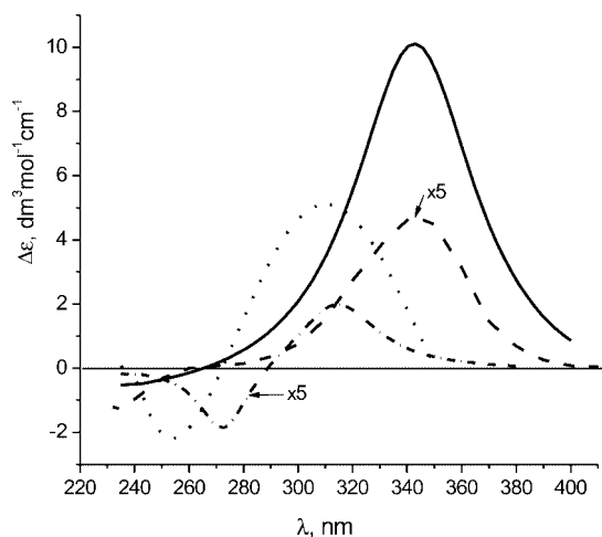
Figure 1. CD spectra of triketone (1 S ,5 R )- 4 (---), ketoenone (1 S ,5 S )- 8 (···), enone (1 S ,5 S )- 7 (—), and bis(enone) (1 S ,5 S )- 9 (— ·) in ethanol.
